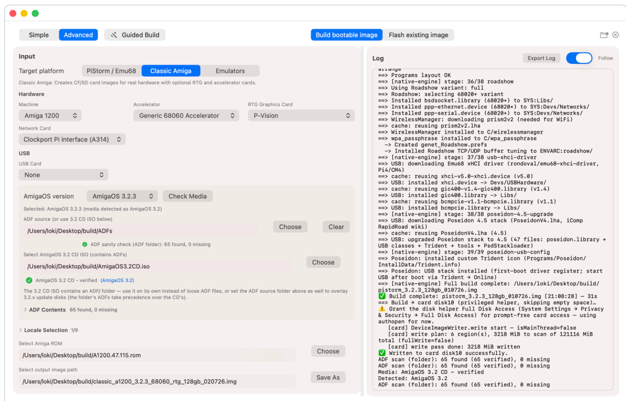
Classic Amiga: machine, accelerator, RTG card, network card, and USB card selectors on the Input card.
